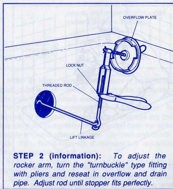
STEP 2: Spring-type bathtub drain has rocker arm that works off lever in overflow plate. This rod can be adjusted so closer seats tightly in the tub strainer. Remove the plate.
